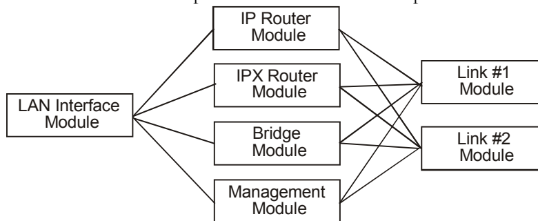
Figure 1 - 1 IOLINK Router Block Diagram
