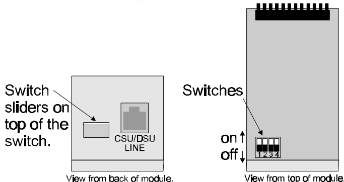
Figure 3 - 2 View of ATL CSU/DSU Link Module with Sliding ON/OFF Switches
