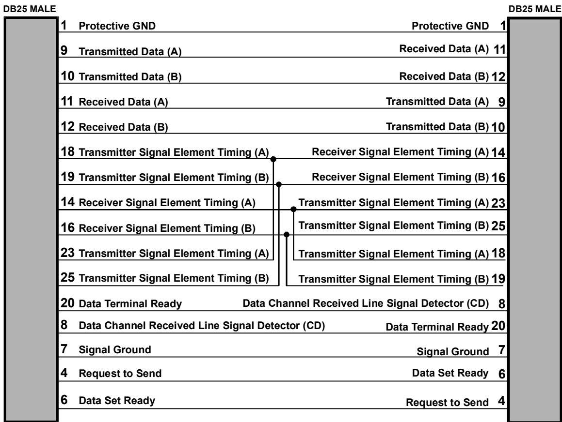
Figure 3 - 10b Early model V.35 Null-Modem Cable
