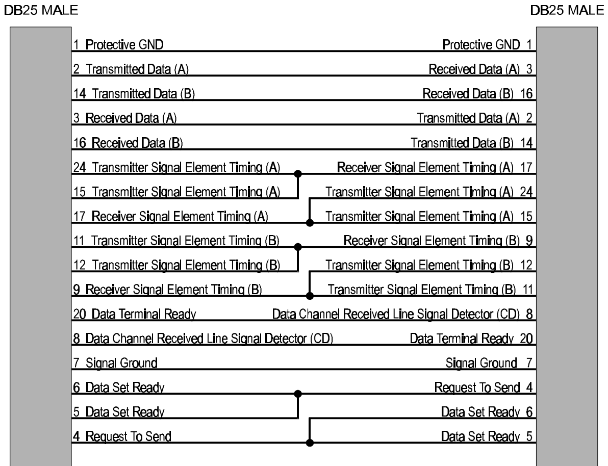
Figure 3 - 10 V.35 Null-Modem Cable
