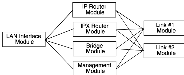
Figure 1 - 1 IOLINK-PRO Ethernet Bridge/Router Block Diagram
