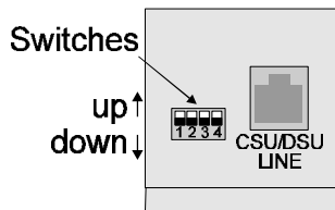
Figure 3 - 1 Rear View of ATL CSU/DSU Link Module with UP/DOWN Switches
