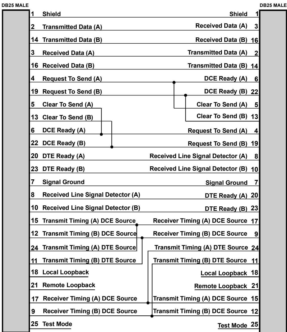
Figure 3 - 11 RS530 Null-Modem Cable
