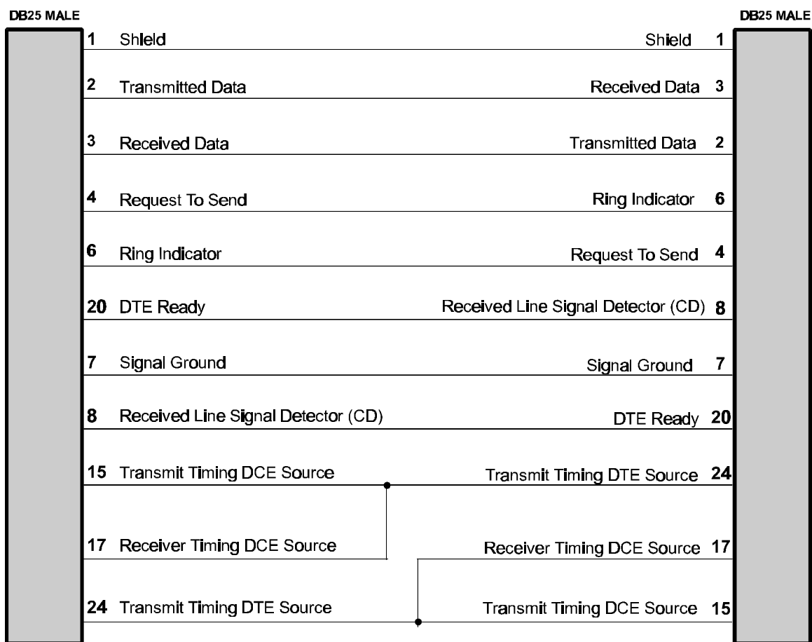
Figure 3 - 9 RS232 Null-Modem Cable
