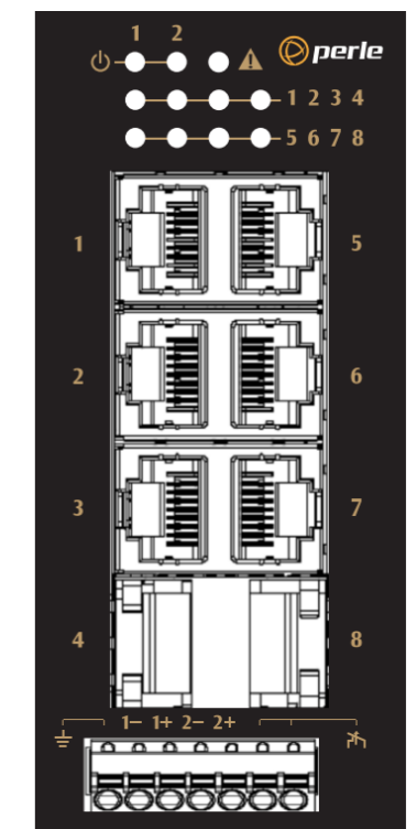
IDS-106F(G)E IDS-106F(G)E-XT
